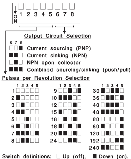
Figure 1 - Configuration Switches
