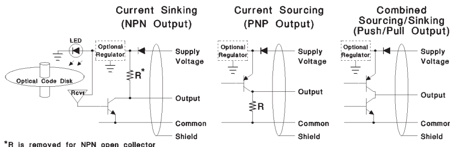
Figure 2 - Output Circuits
